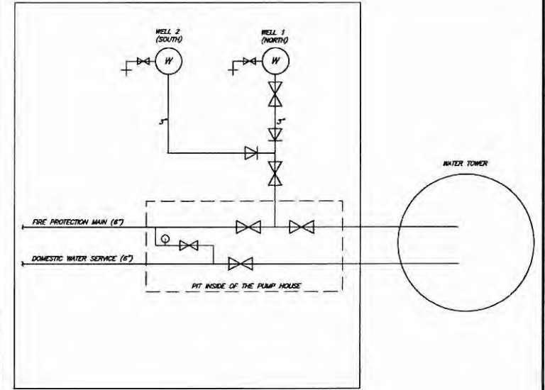
PUMP HOUSE
