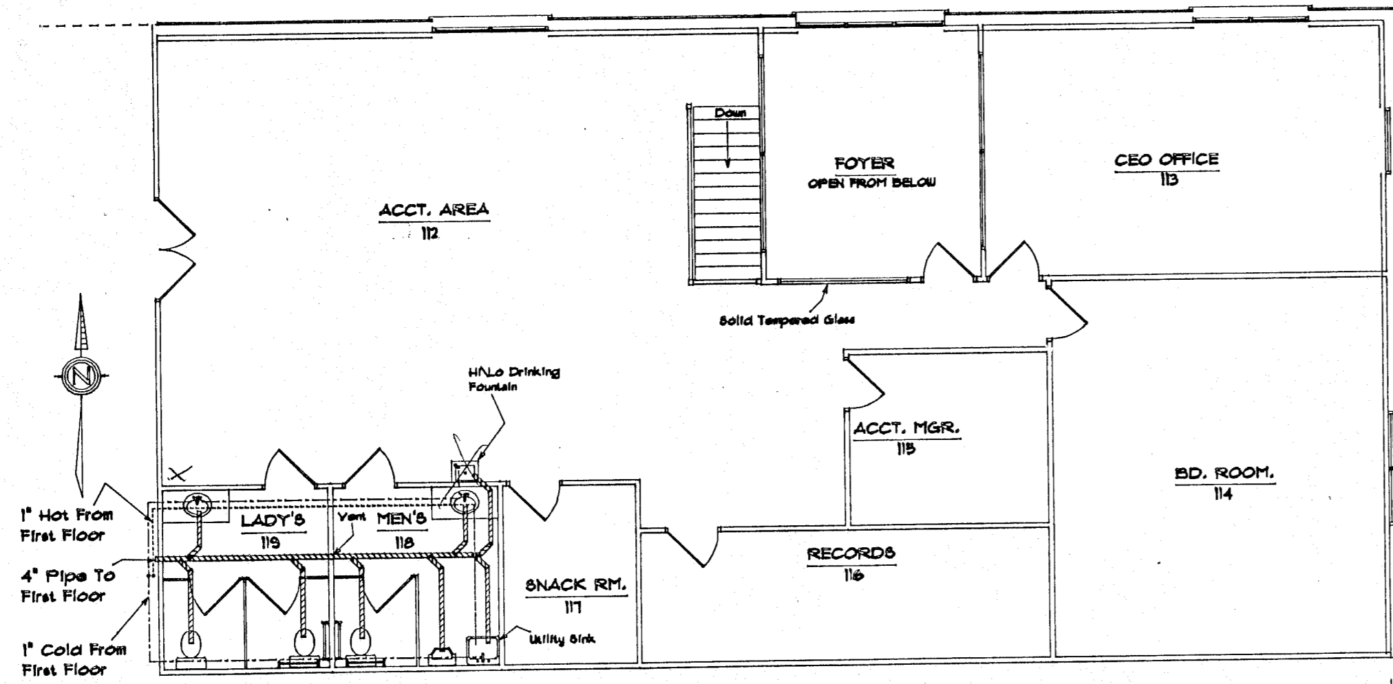
UPPER FLOOR PLUMBING
