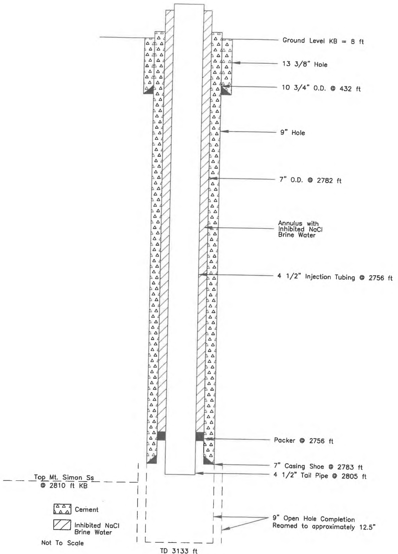
FIGURE 2-4 WELL SCHEMATIC OF INEOS WDW NO.1 AS OF DECEMBER 2021
